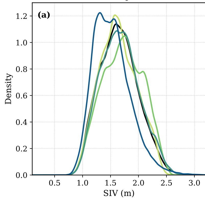
Winter (JFM)
