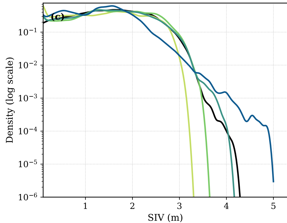
Annual
