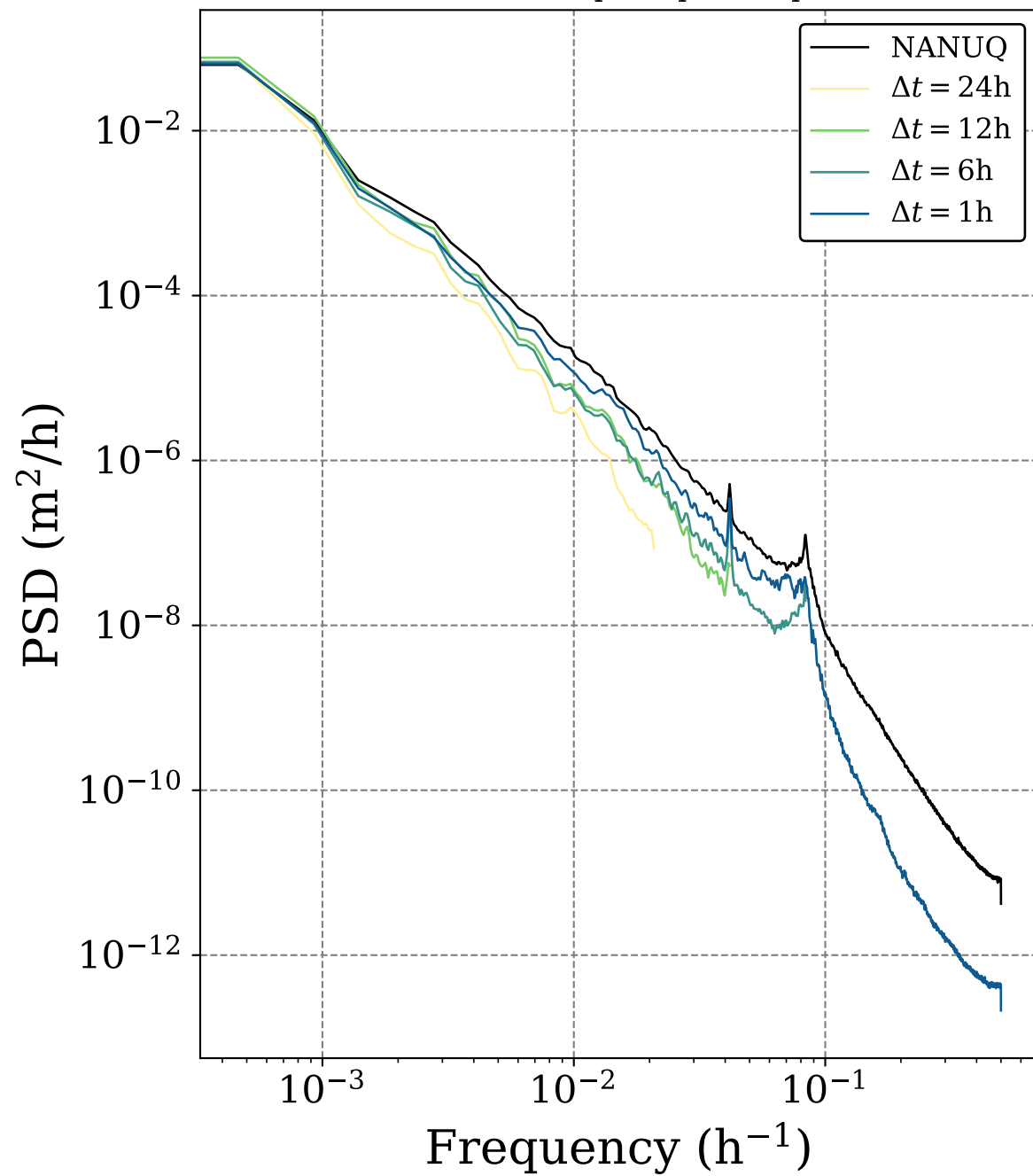
Central Arctic temporal power spectrum
