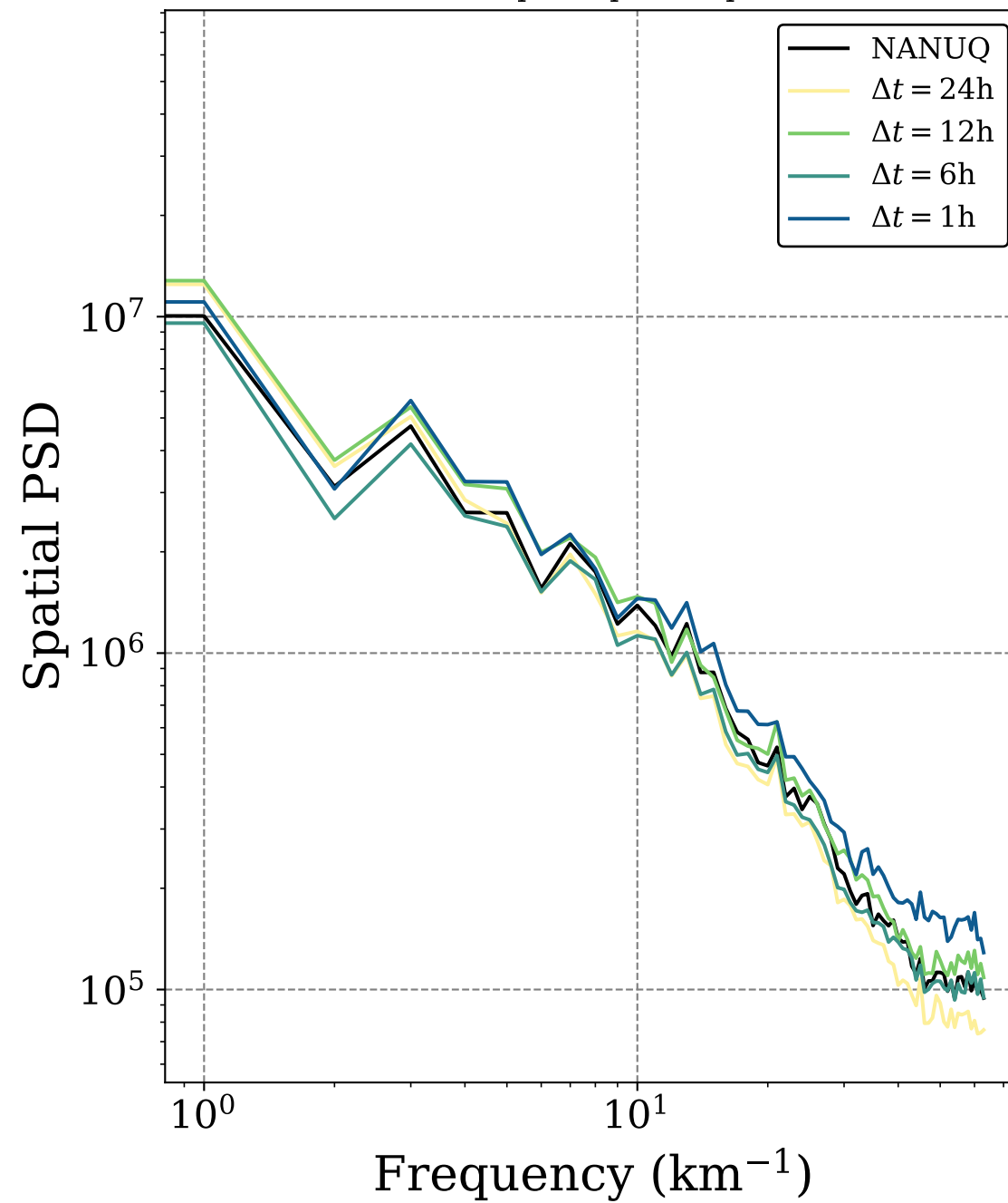
Full Arctic spatial power spectrum
