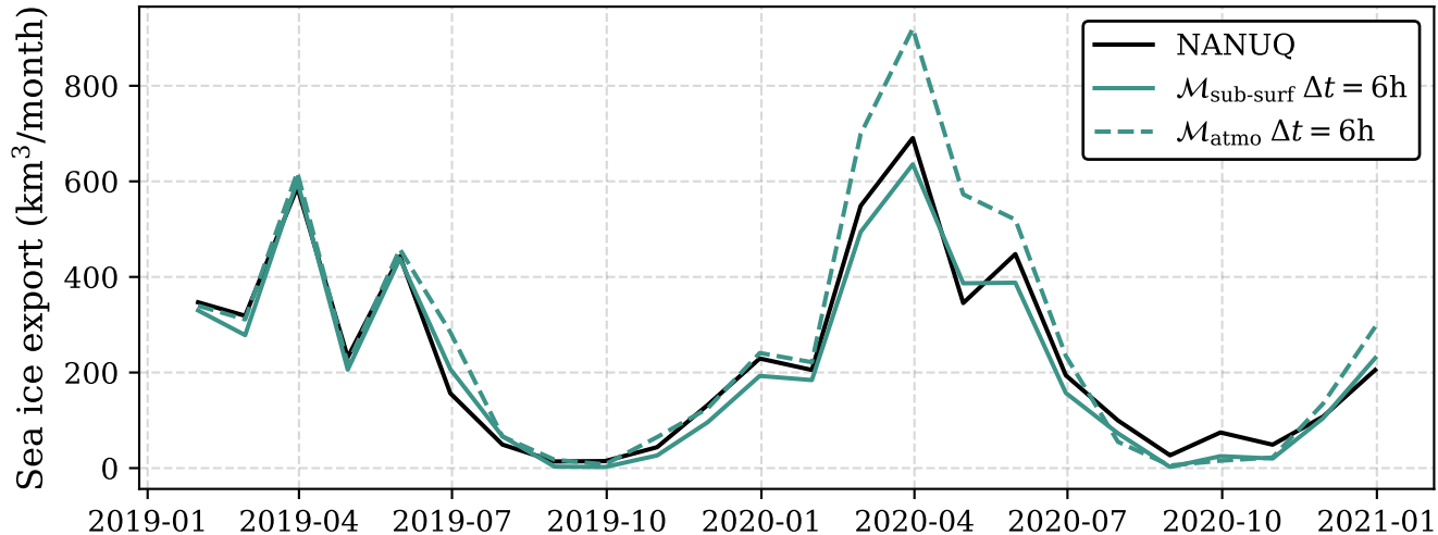
Fram Strait monthly export
