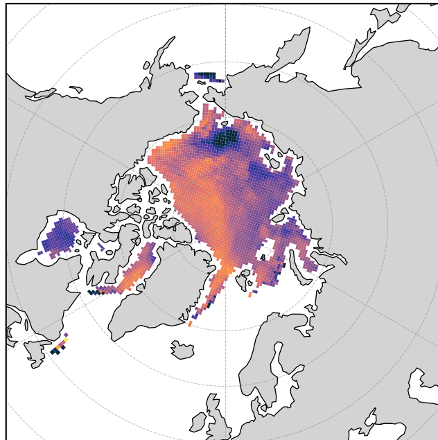
\mathcal{M}_{\text{sub-surf}} ERA5
