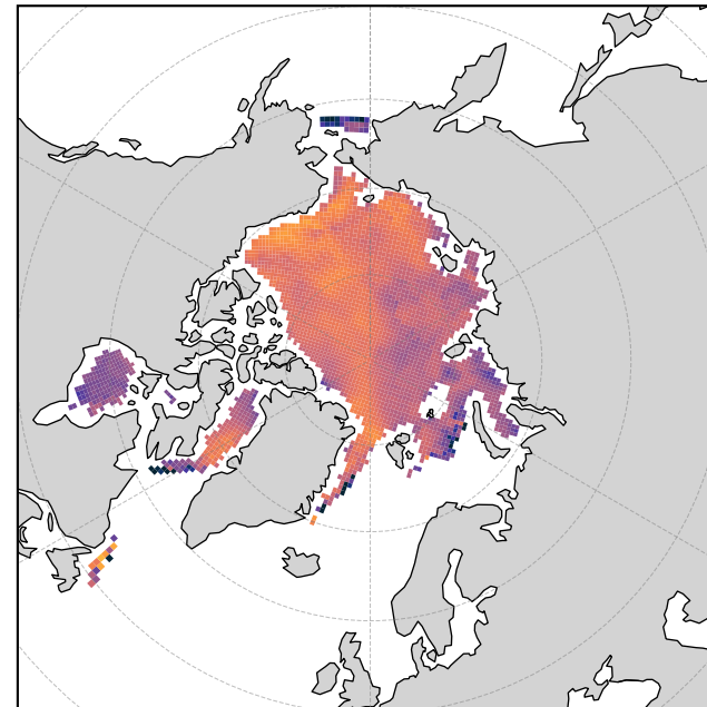
\mathcal{M}_{\text{red}} JRA55
