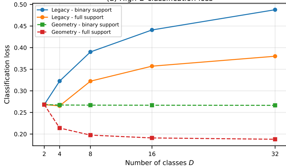
(a) High-D classification loss
