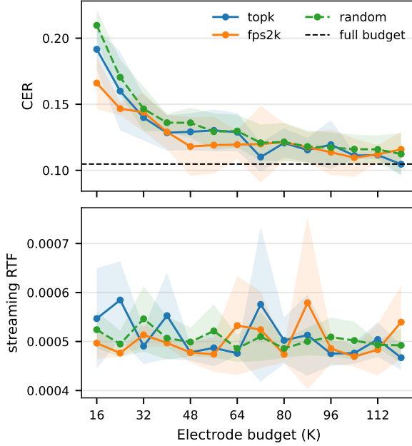
Figure 1: Electrode-budget trends for P1 word hold-out; topk uses within-participant importance ranking, diversity corresponds to fps2k, and random is a fixed random subset. CER is character error rate and RTF is real time factor.
