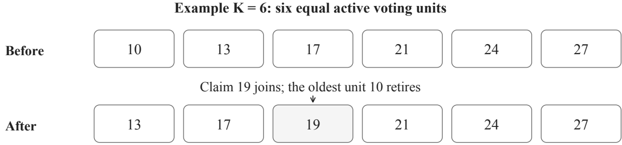
Figure 8. In this six-unit illustration, unused contribution 19 qualifies because it is newer than the oldest installed contribution, 10. A successful installation replaces 10 and places 19 in its original contribution order. This example shows the replacement arithmetic; ownership of the six units is a separate matter.
