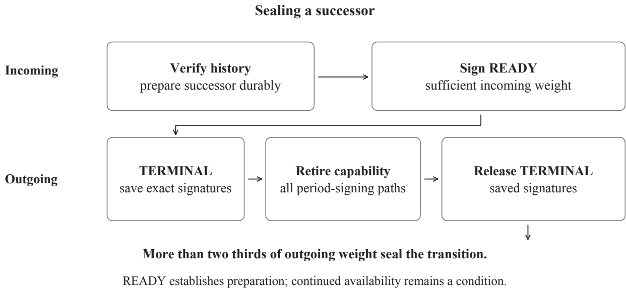
Figure 9. Preparation precedes READY. Saved TERMINAL signatures are released only after signing capabilities are retired; the outgoing seal authorizes the next height.
