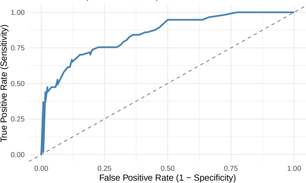
ROC Curve (AUC = 0.8489 )
