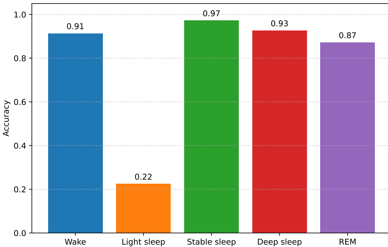
LSTM
