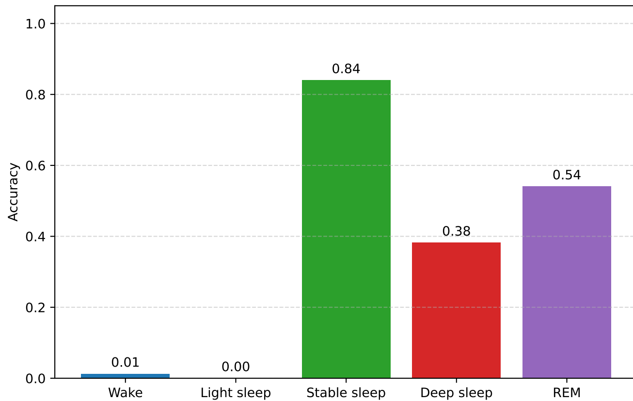
Attention
