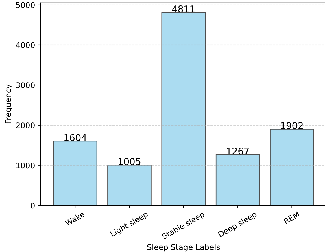
Sleep Stage Label Distribution (Training)
