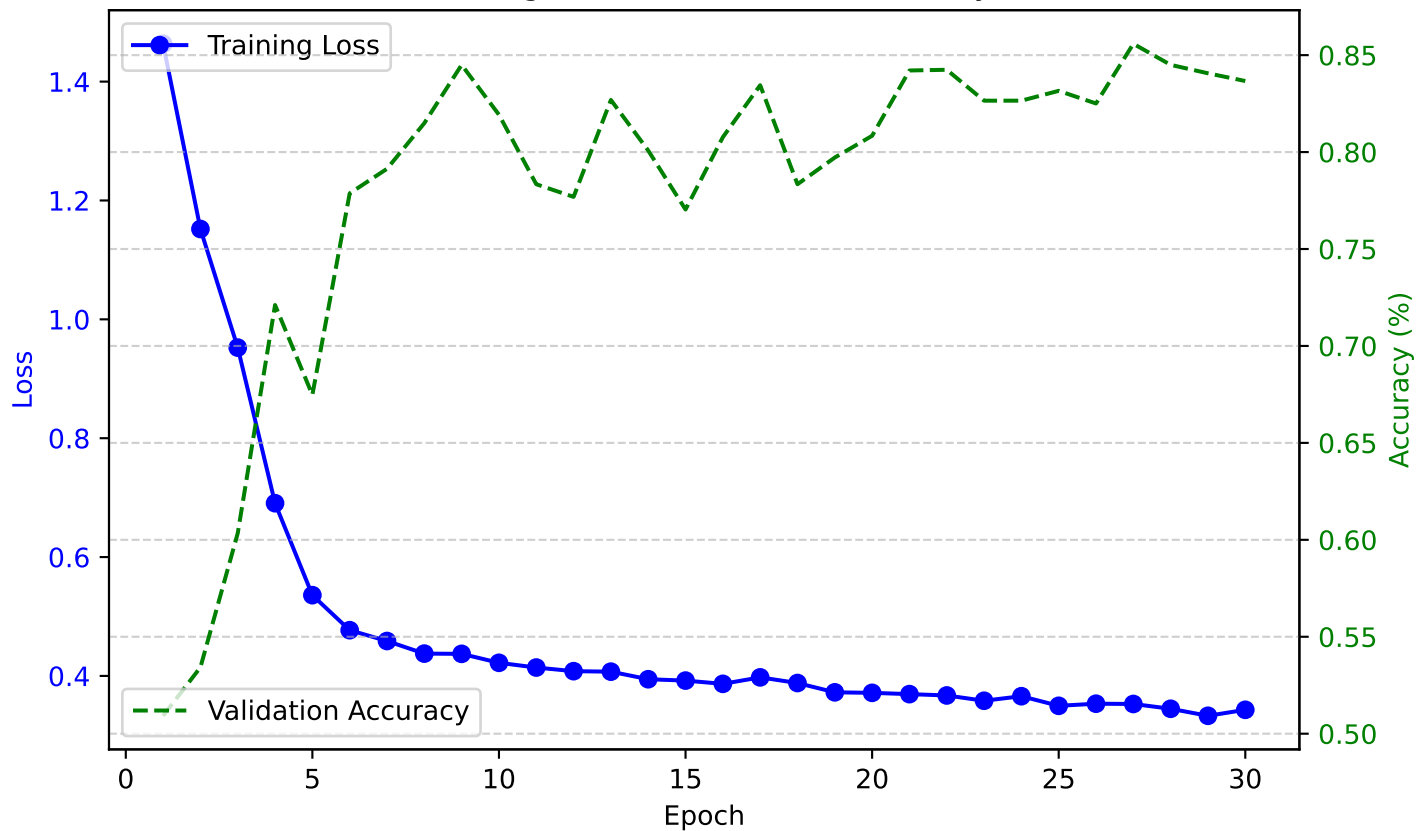
Training Loss vs Validation Accuracy
