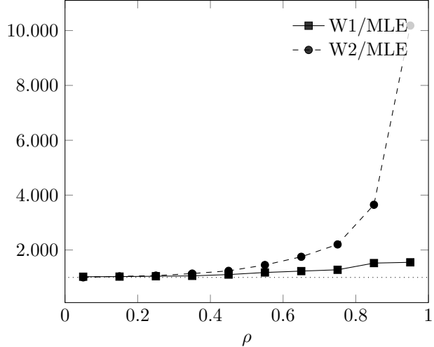
\mu MSE ratio w.r.t. MLE
