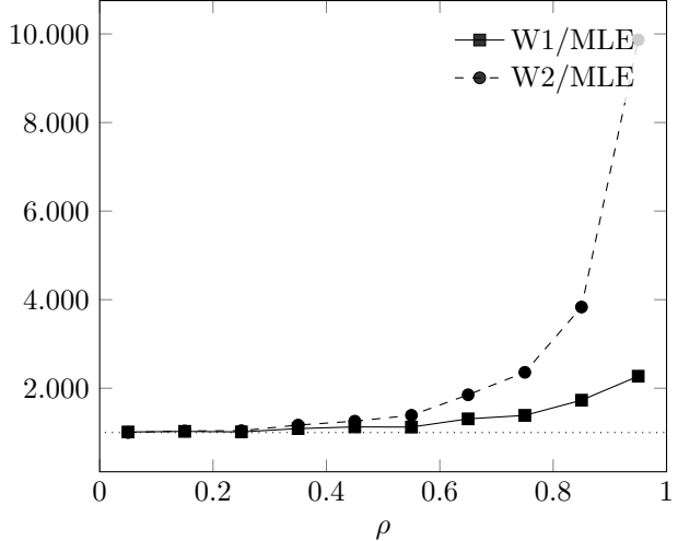
\rho MSE ratio w.r.t. MLE
