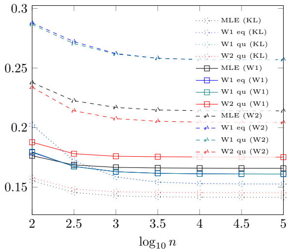
Distance to true
