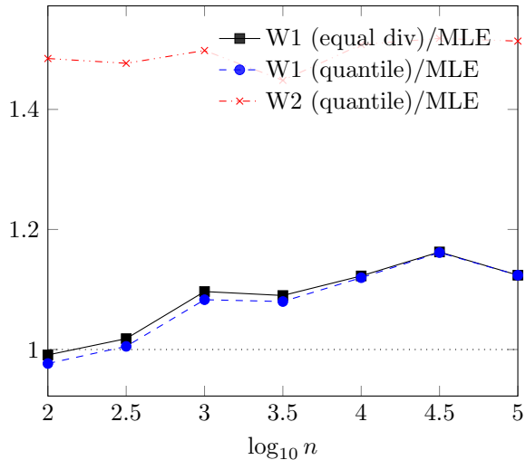
\mu MSE ratio w.r.t. MLE
