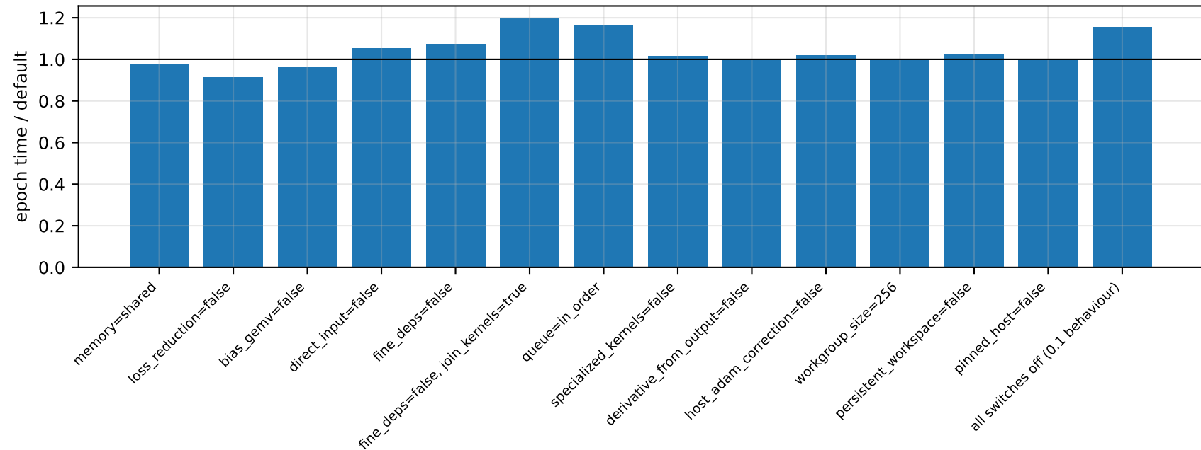
syncInn ablations - cup (float, b=40) on TR 2950X
