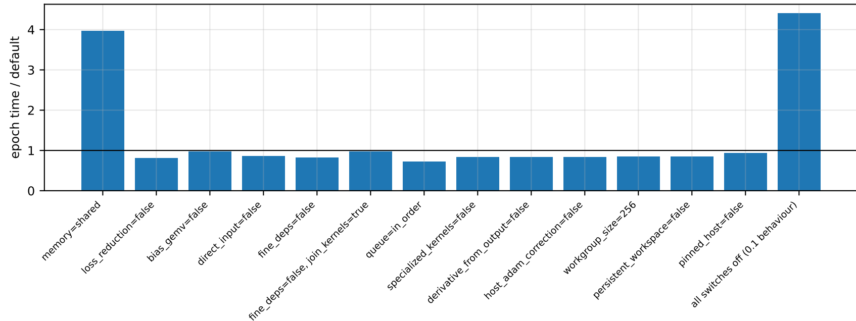
syclnn ablations - mnist-512-256 (float, b=256) on RX 7900 XTX
