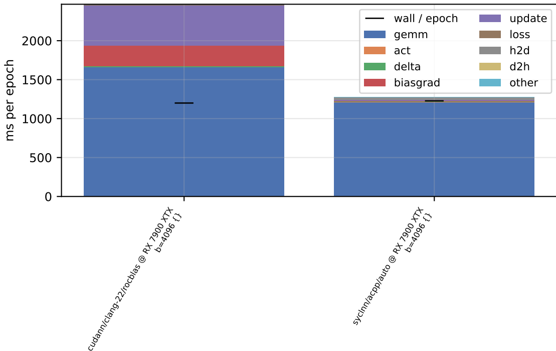
per-phase device time - sweep-w1024-d4-b4096 (double, train)
