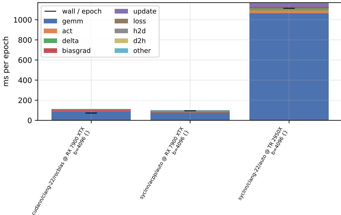
per-phase device time - sweep-w1024-d4-b4096 (float, train)
