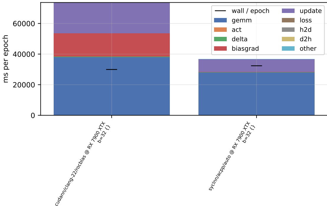
per-phase device time - sweep-w4096-d4-b32 (double, train)
