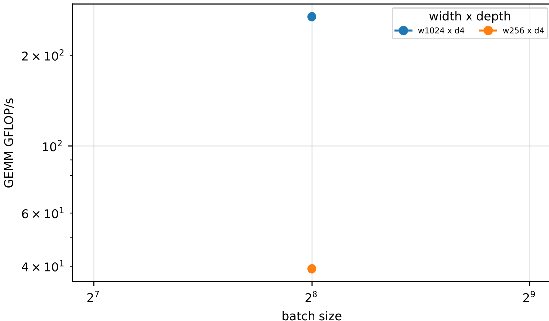
W4 sweep - ompnn/gcc-14/rocblas @ RX 7900 XTX (float)
