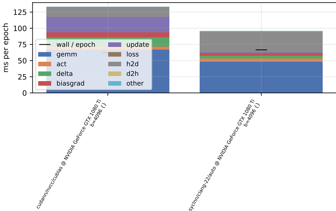
per-phase device time - sweep-w1024-d2-b4096 (float, train)
