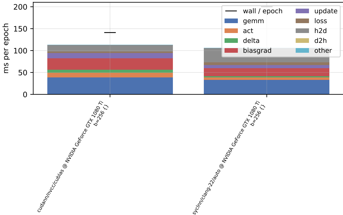
per-phase device time - sweep-w256-d2-b256 (float, train)
