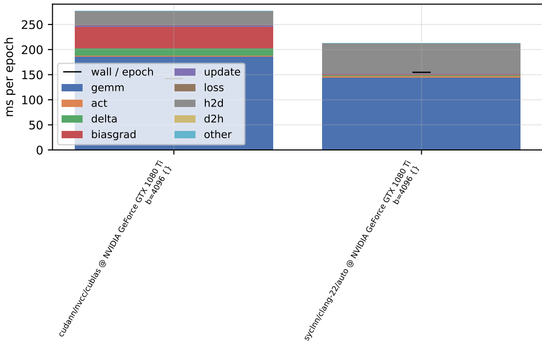
per-phase device time - sweep-w256-d2-b4096 (double, train)
