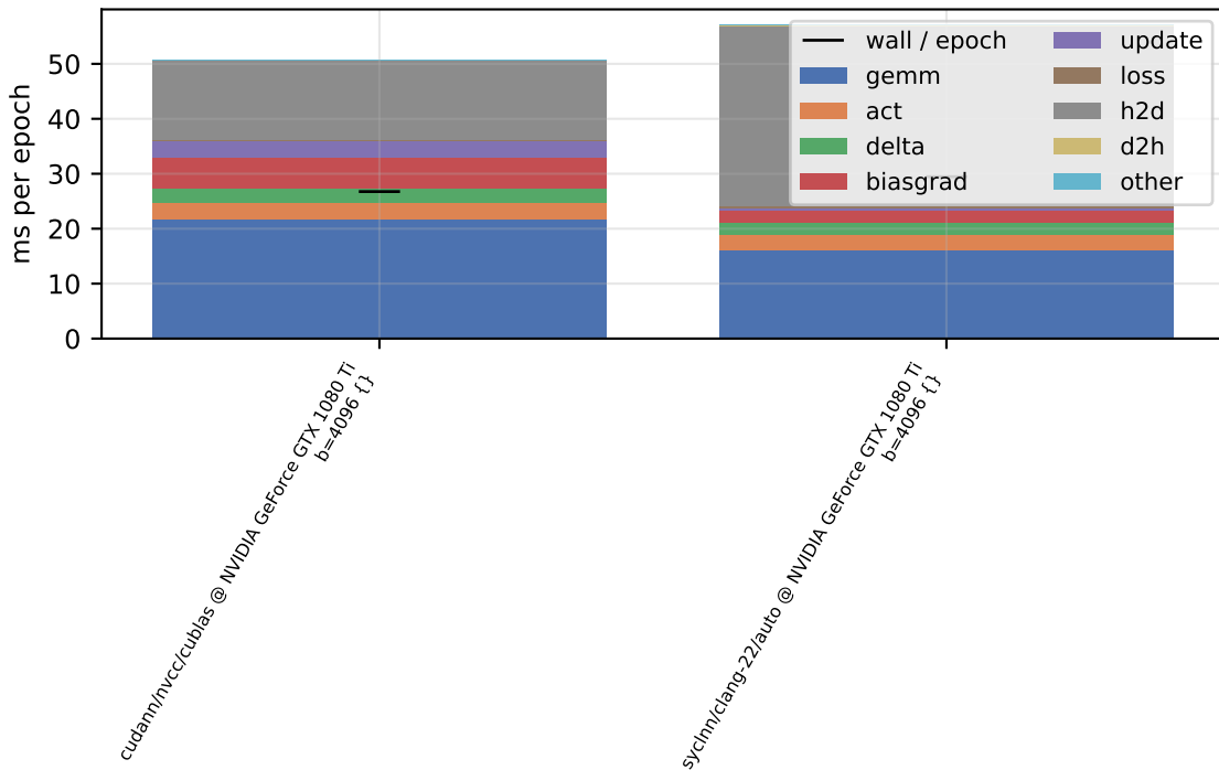
per-phase device time - sweep-w256-d4-b4096 (float, train)
