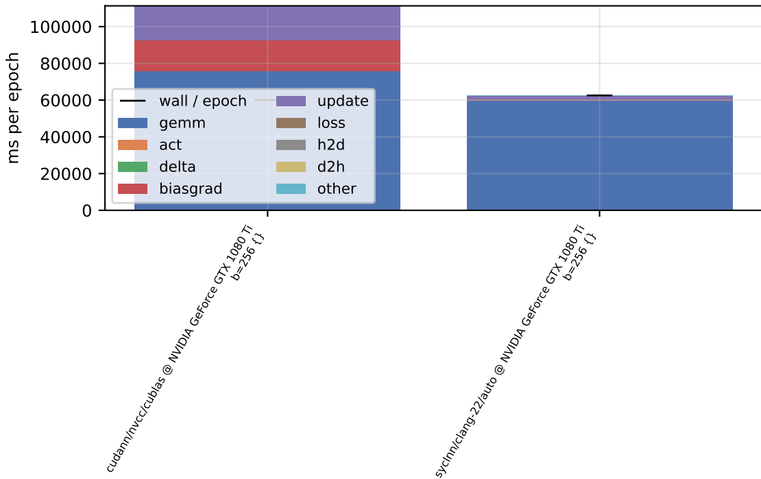
per-phase device time - sweep-w4096-d4-b256 (double, train)
