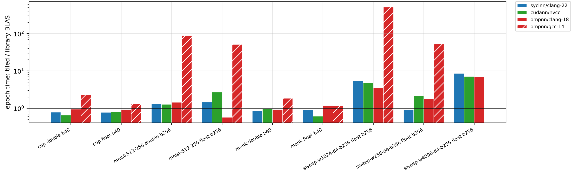
hand-written 16x16 tiled GEMM vs library on NVIDIA GeForce GTX 1080 Ti
