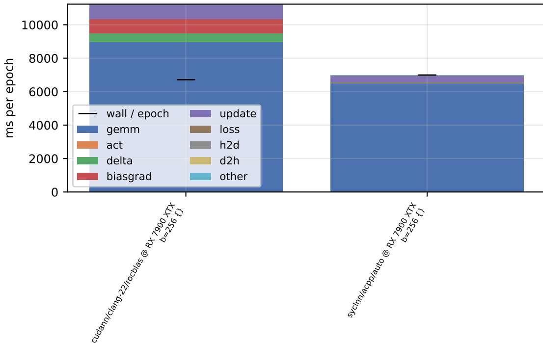
per-phase device time - sweep-w4096-d2-b256 (double, train)
