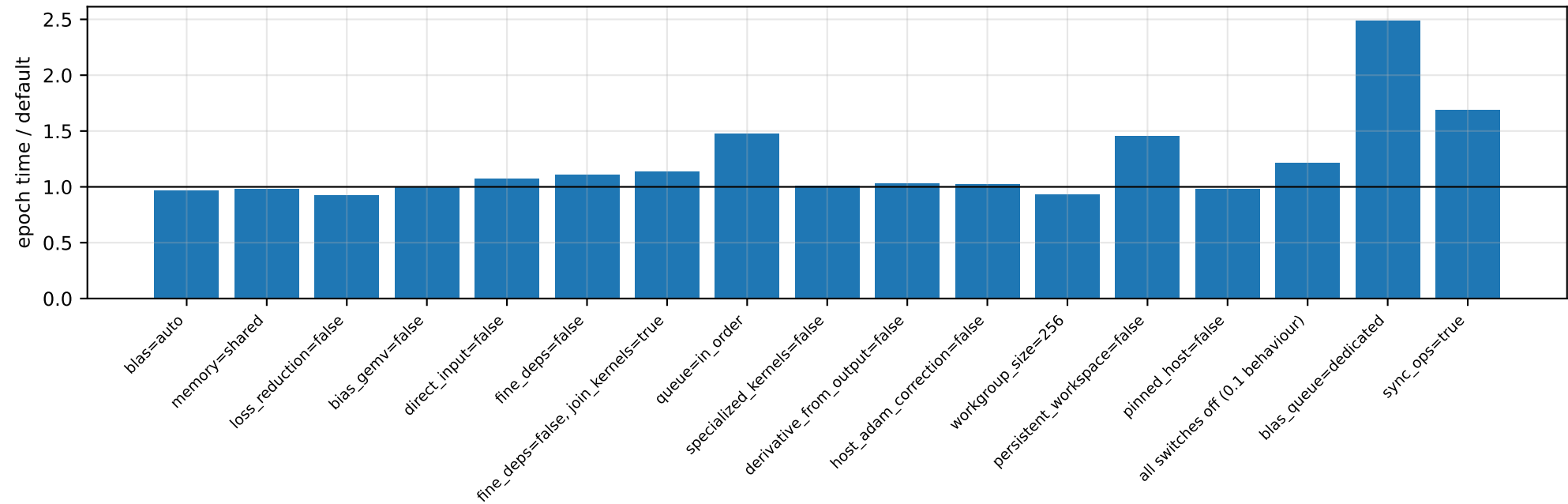
syclnn ablations - cup (float, b=40) on TR 2950X
