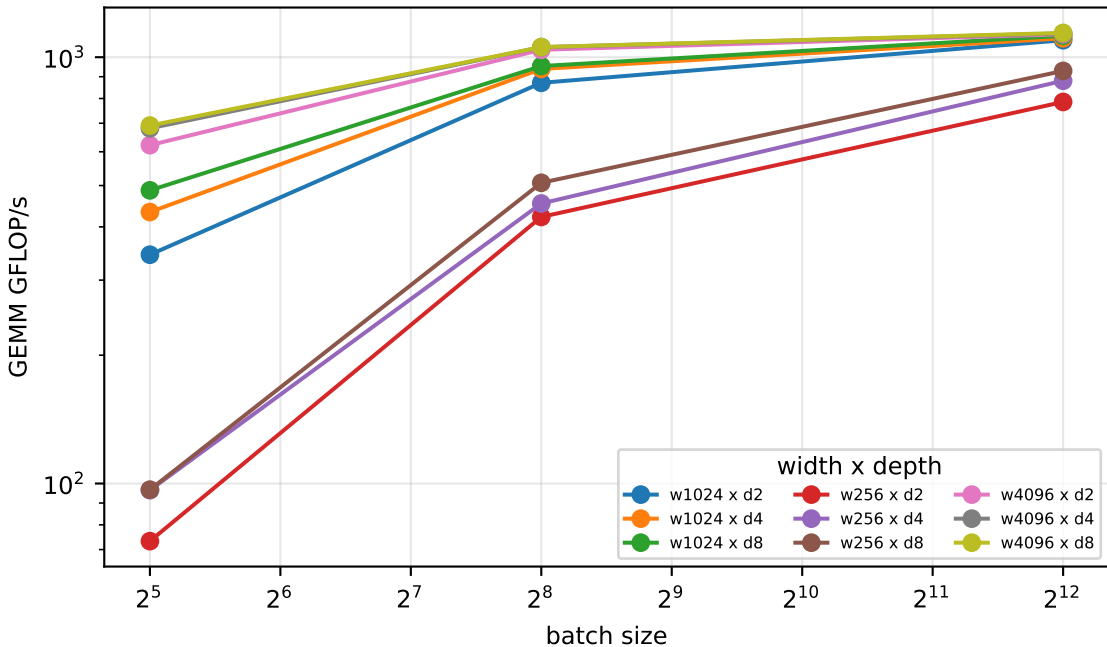
W4 sweep - cudann/clang-22/rocblas @ RX 7900 XTX (double)
