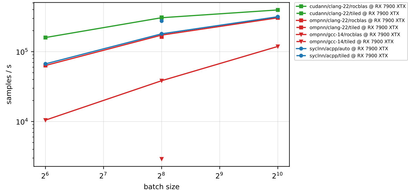
training throughput - mnist-512-256 (double, gpu)
