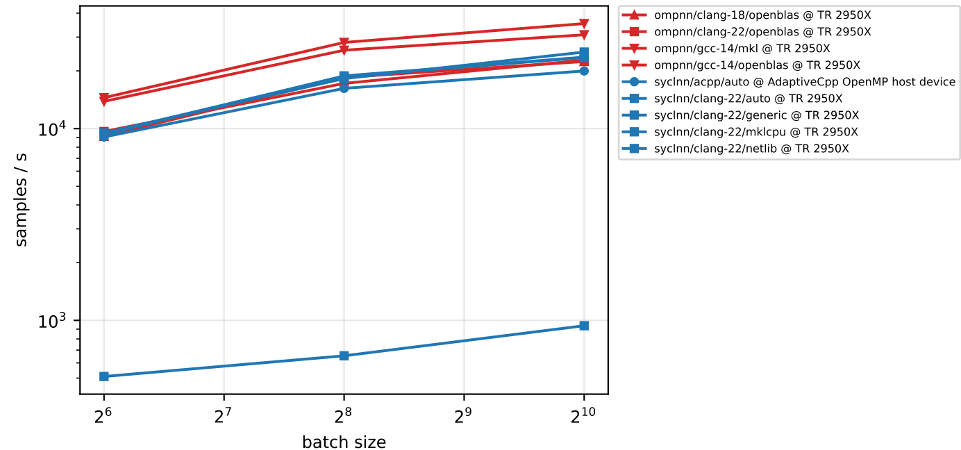
training throughput - mnist (float, cpu)
