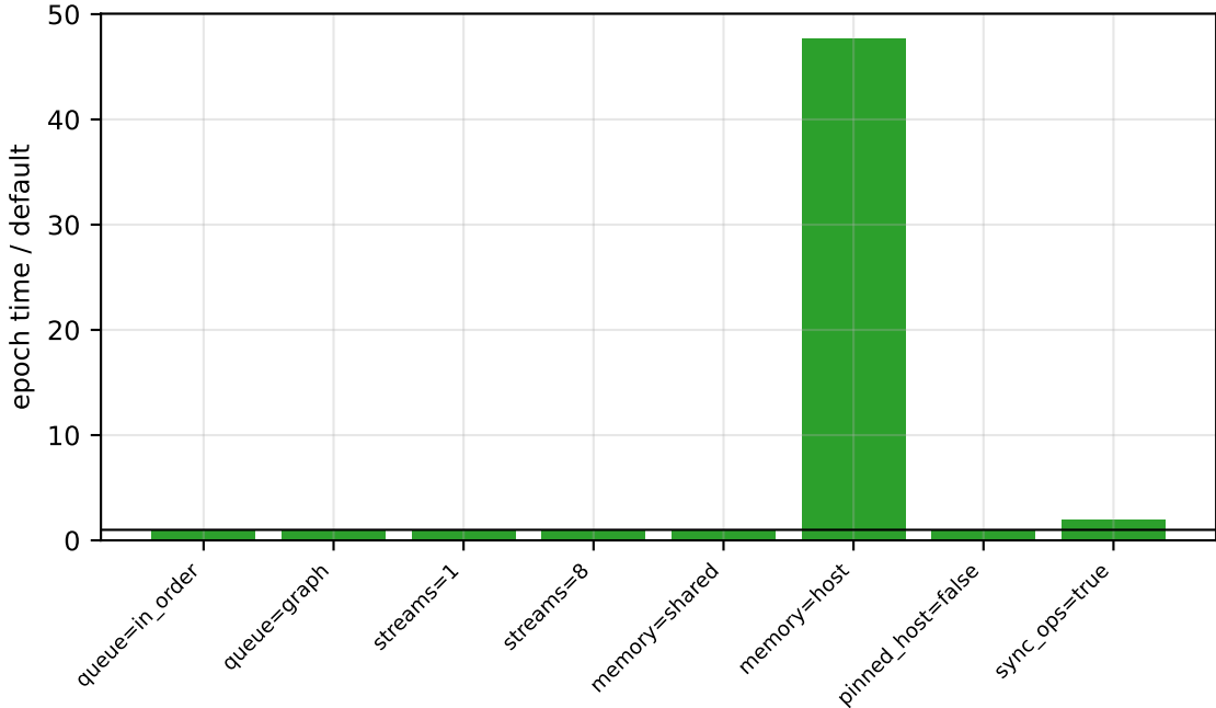
cuda nn ablations - mnist-512-256 (float, b=256) on NVIDIA GeForce GTX 1080 Ti
