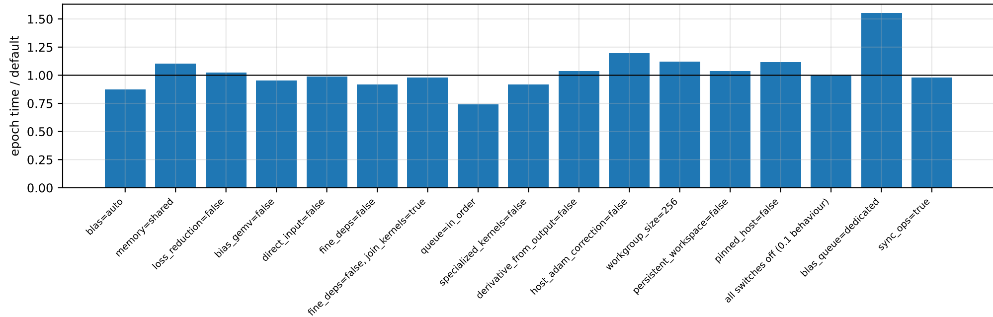
syclInn ablations - mnist-512-256 (float, b=256) on NVIDIA GeForce GTX 1080 Ti
