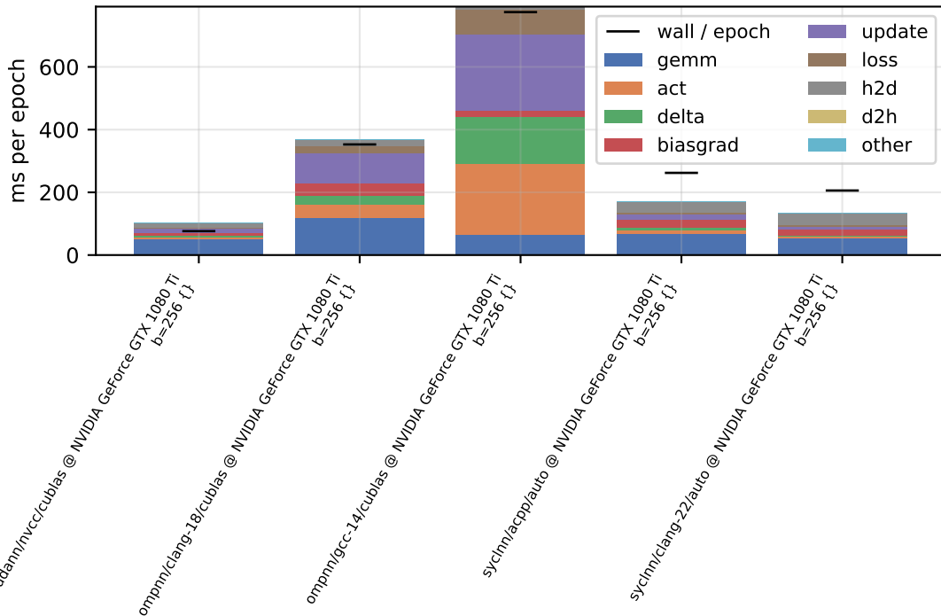
per-phase device time - mnist-512-256 (float, train)
