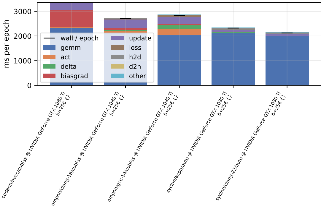
per-phase device time - mnist (double, train)
