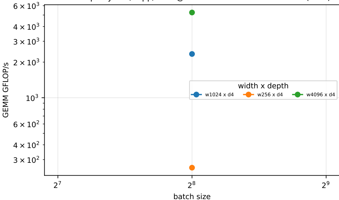
W4 sweep - syclInn/acpp/auto @ NVIDIA GeForce GTX 1080 Ti (float)
