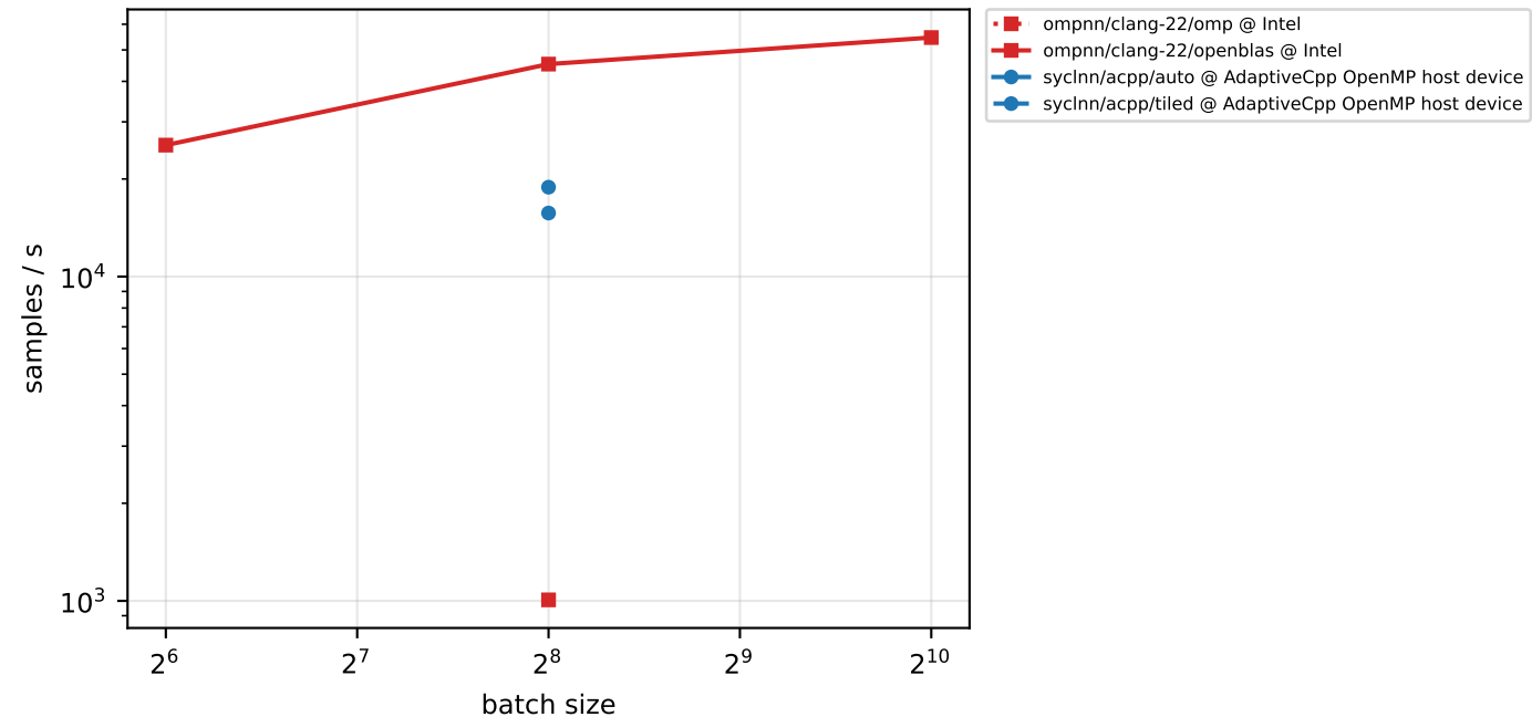
training throughput - mnist-512-256 (float, cpu)
