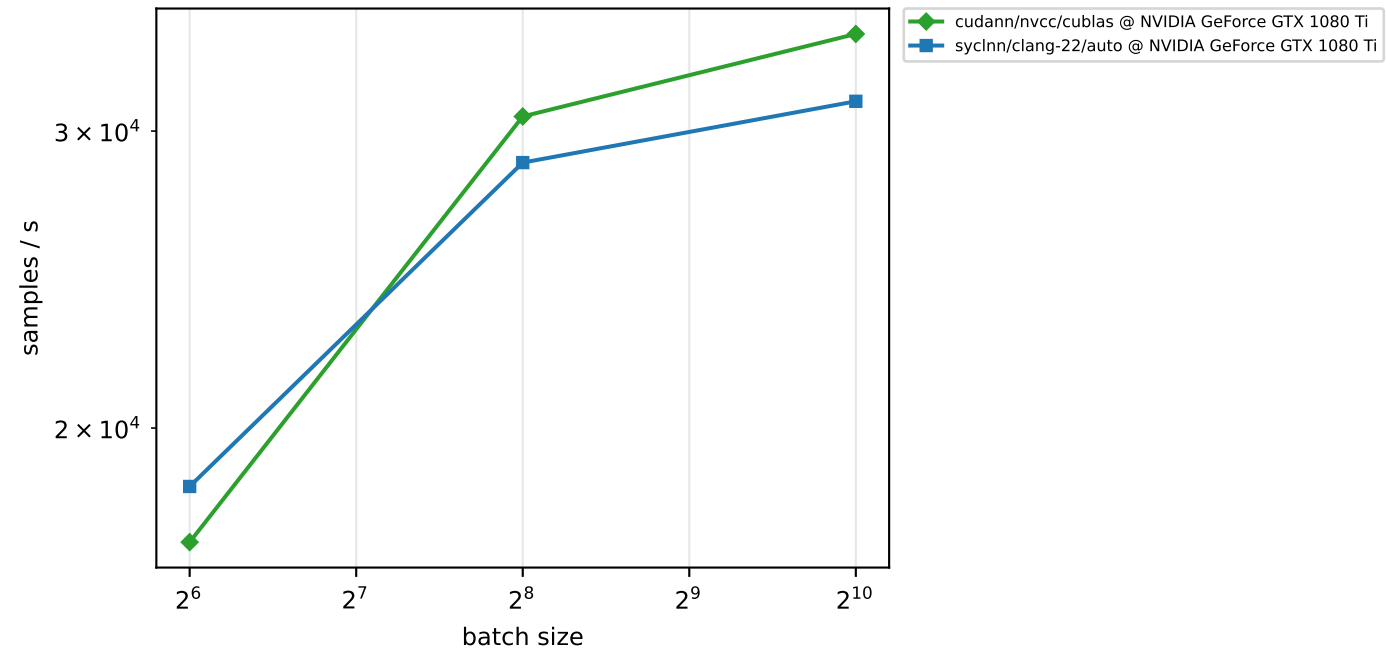
training throughput - mnist (double)
