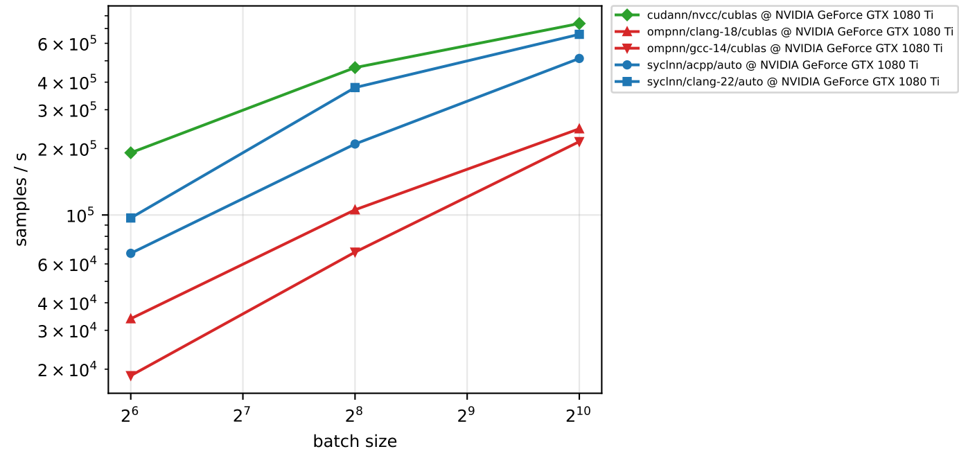
training throughput - mnist (float, gpu)
