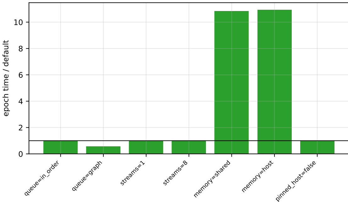
cudaann ablations - mnist-512-256 (float, b=256) on RX 7900 XTX
