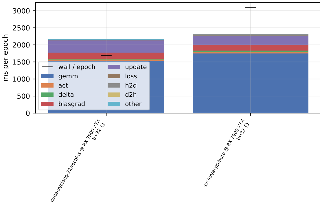
per-phase device time - sweep-w1024-d2-b32 (double, train)
