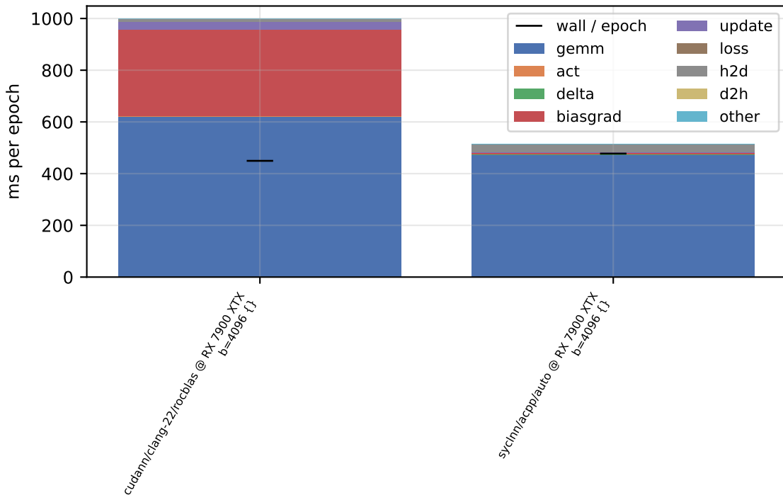
per-phase device time - sweep-w1024-d2-b4096 (double, train)
