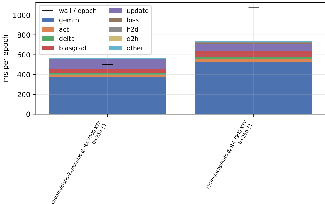
per-phase device time - sweep-w1024-d8-b256 (float, train)
