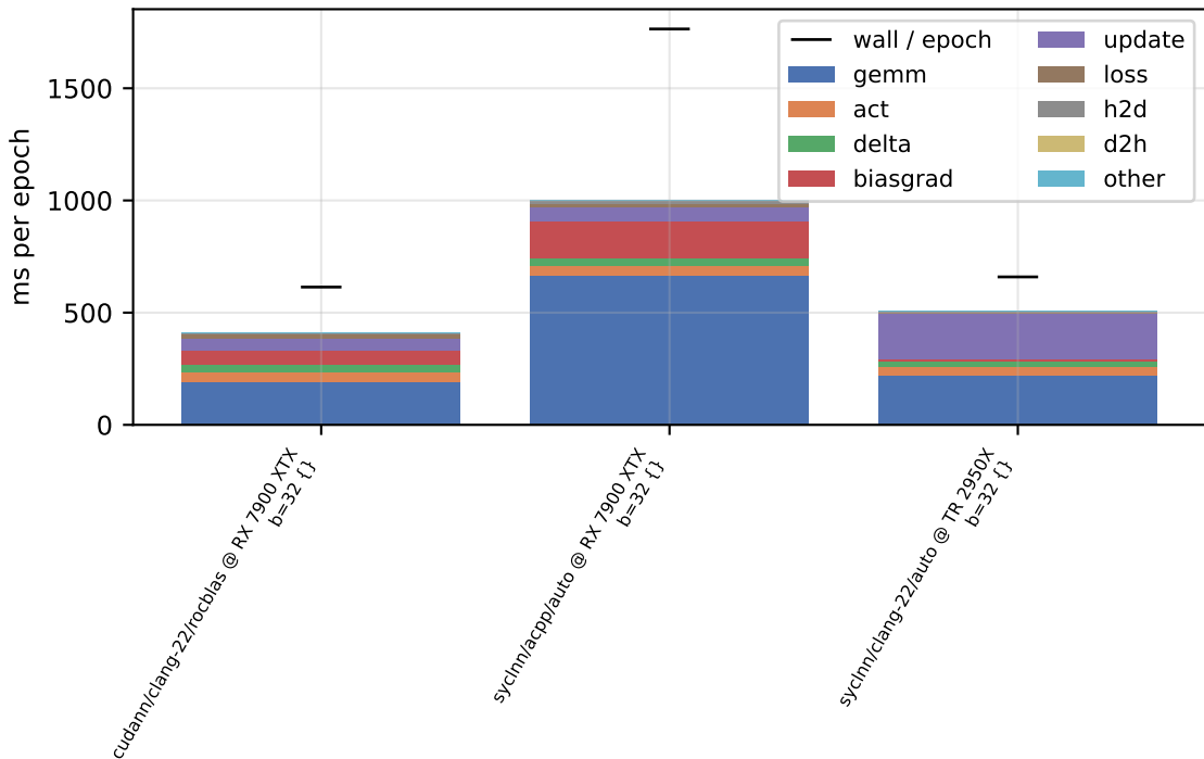
per-phase device time - sweep-w256-d2-b32 (float, train)
