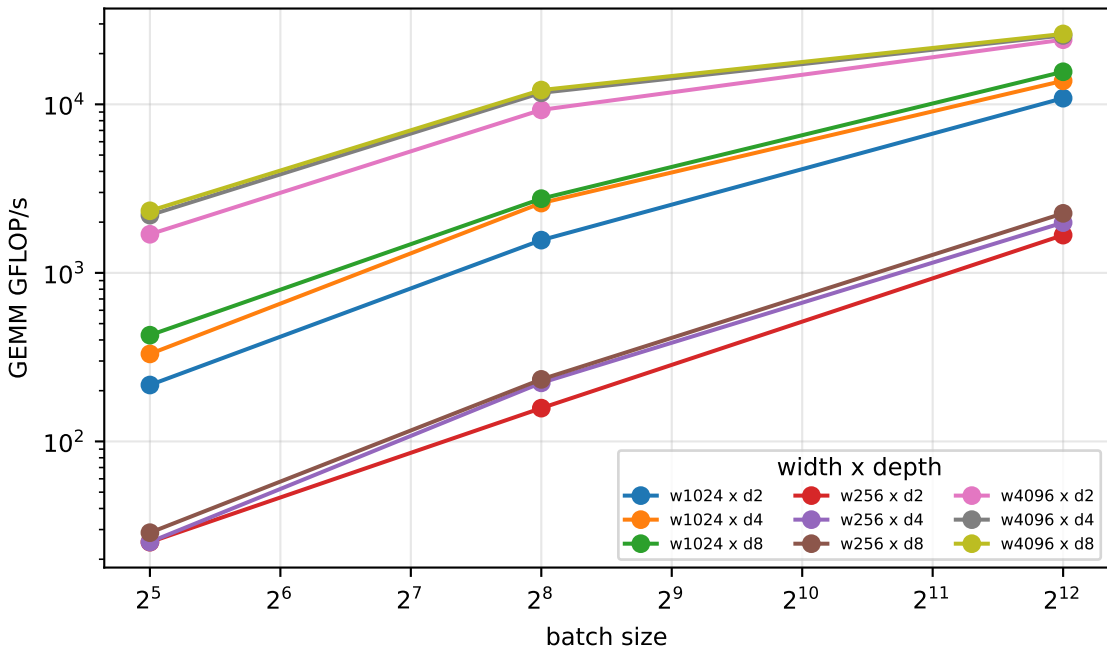
W4 sweep - syclinn/acpp/auto @ RX 7900 XTX (float)
