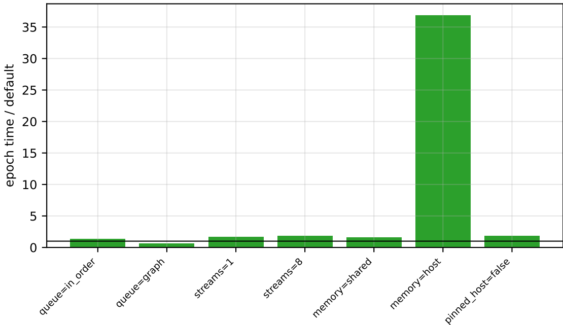
cudaann ablations - mnist-512-256 (float, b=256) on NVIDIA GeForce GTX 1080 Ti
