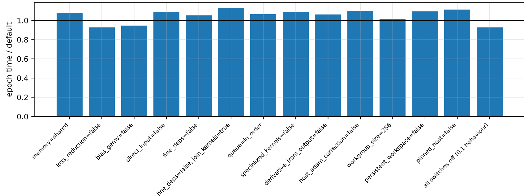
syclnn ablations - mnist-512-256 (float, b=256) on NVIDIA GeForce GTX 1080 Ti
