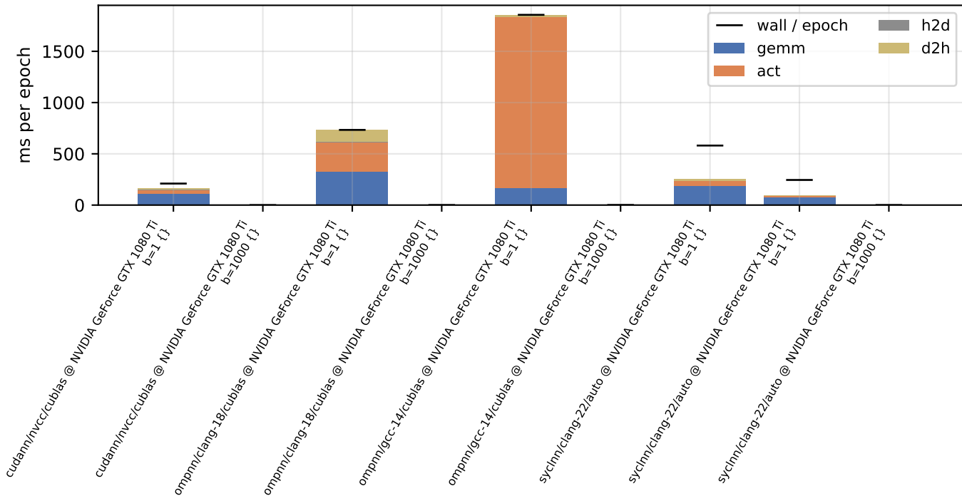
per-phase device time - cup (float, infer)
