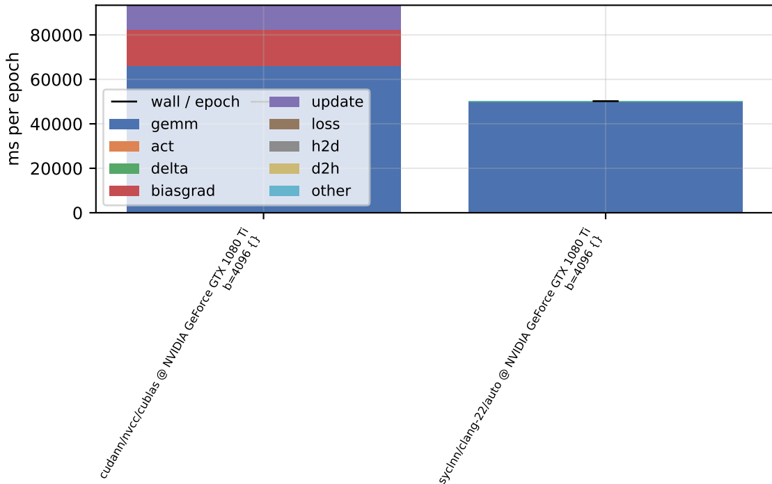
per-phase device time - sweep-w4096-d4-b4096 (double, train)
