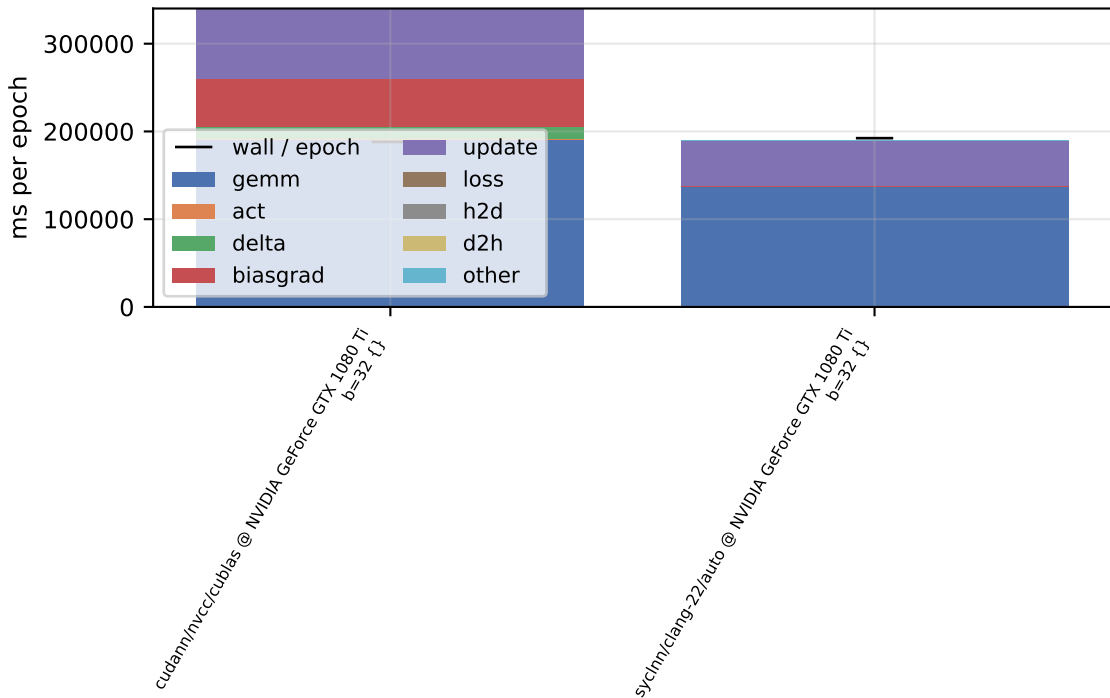
per-phase device time - sweep-w4096-d8-b32 (double, train)
