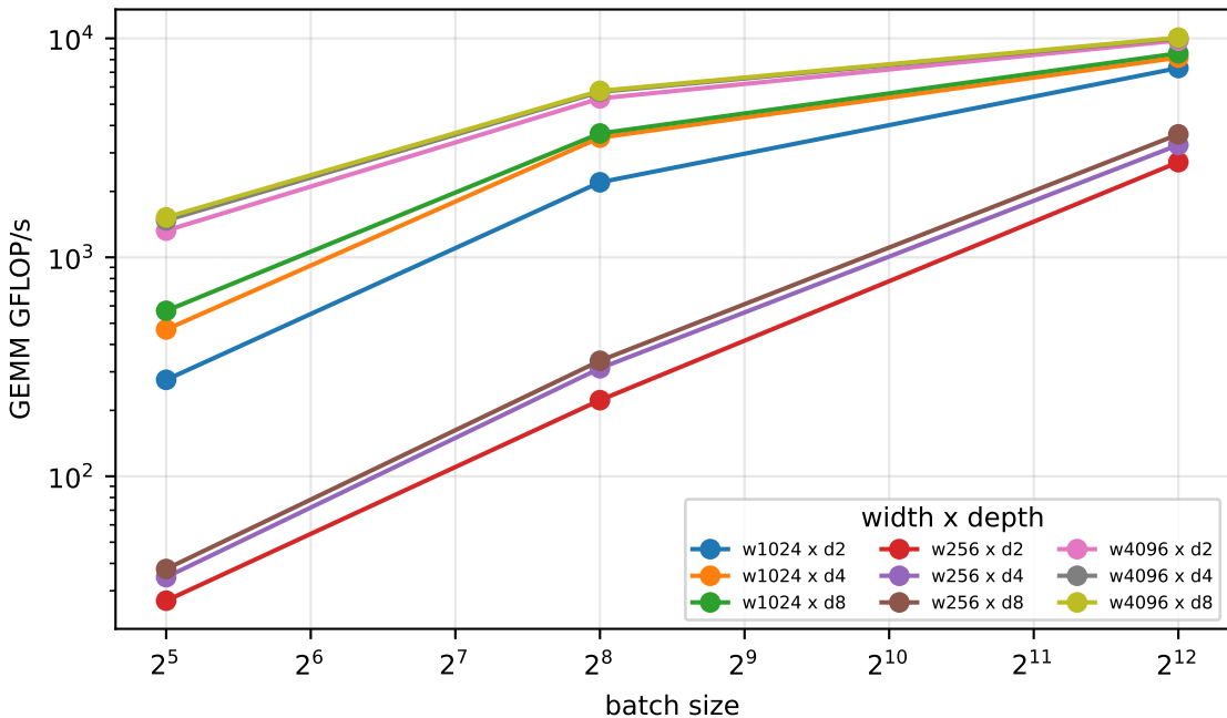
W4 sweep - syclnn/clang-22/auto @ NVIDIA GeForce GTX 1080 Ti (float)
